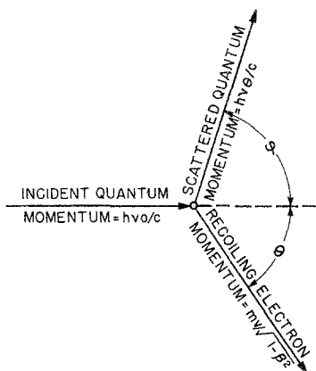
FIG. 1. Recoil of an electron upon scattering of an x-ray photon.
